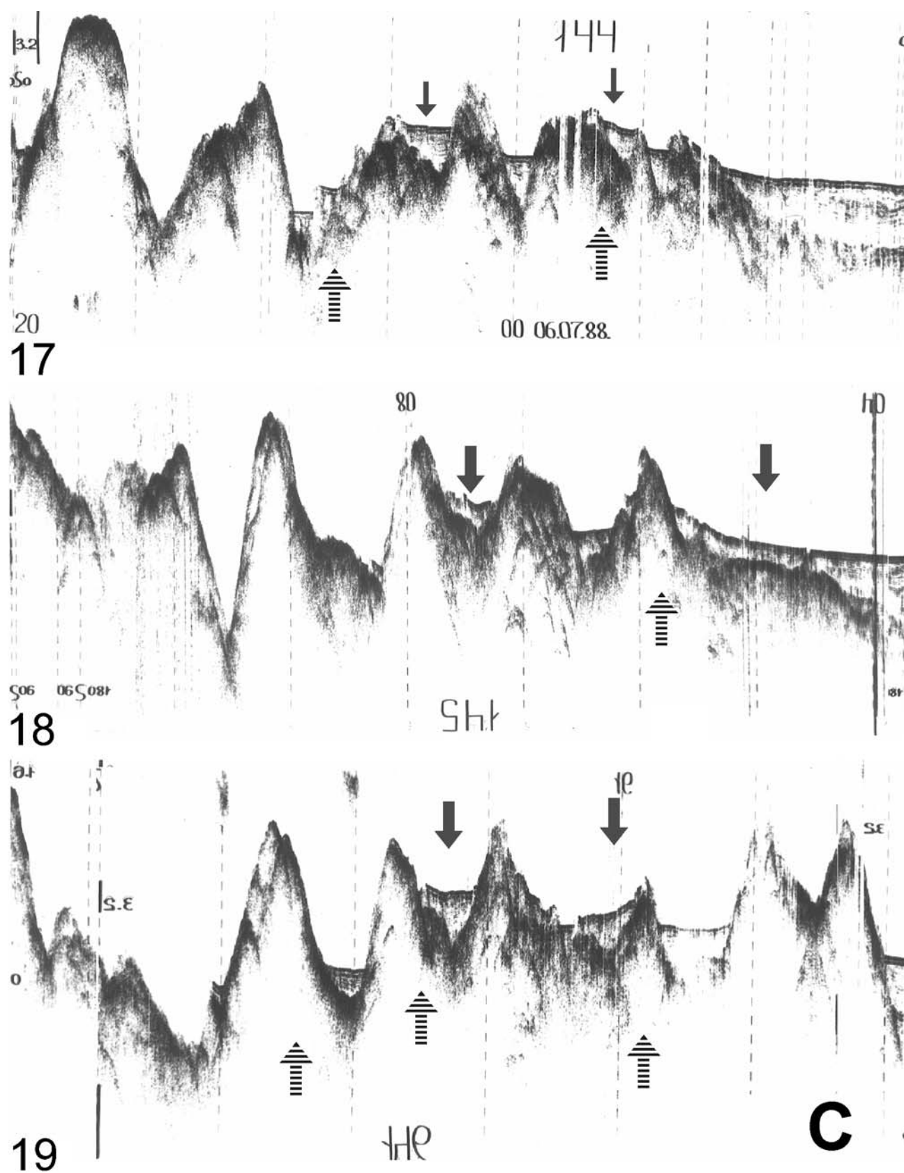
Figure 13. Continuation. c – Seismic profiles 17–19.
