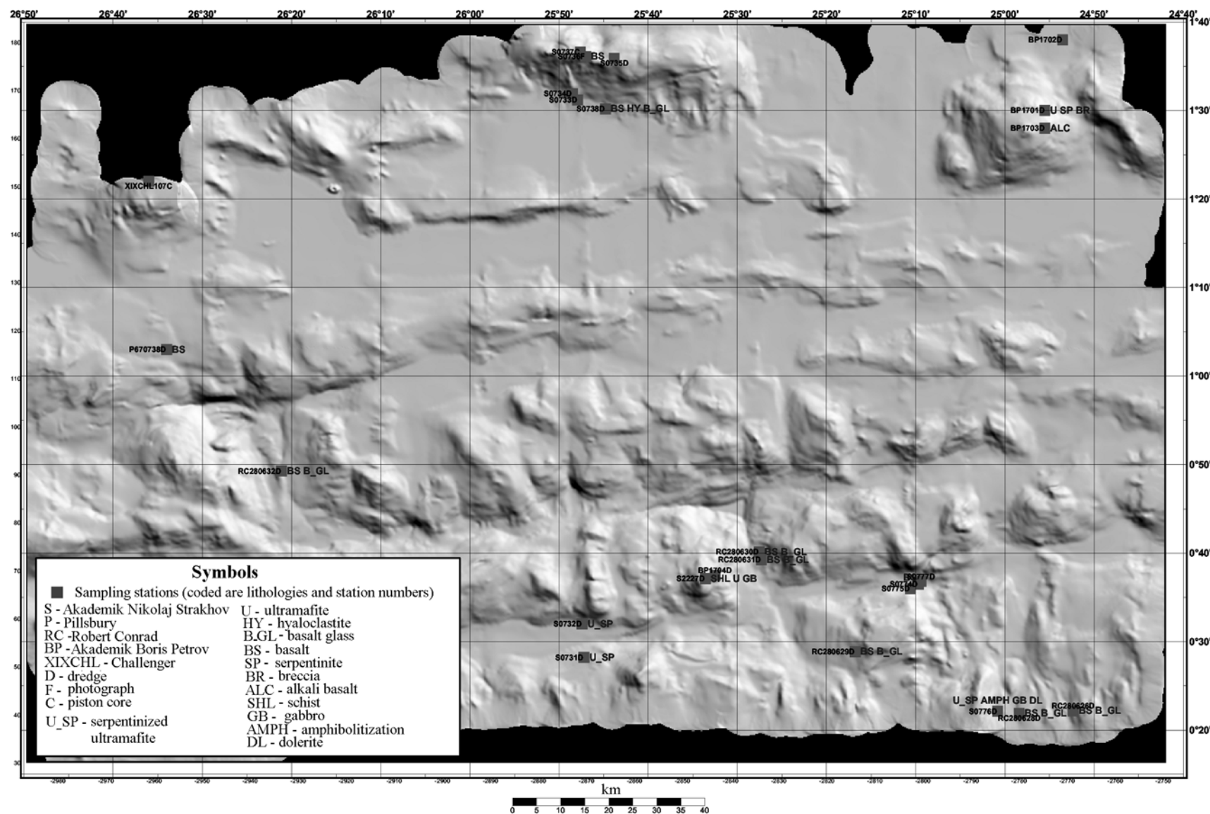
Figure 11. Bedrock geology of the active segment of the São Paulo FZ.
