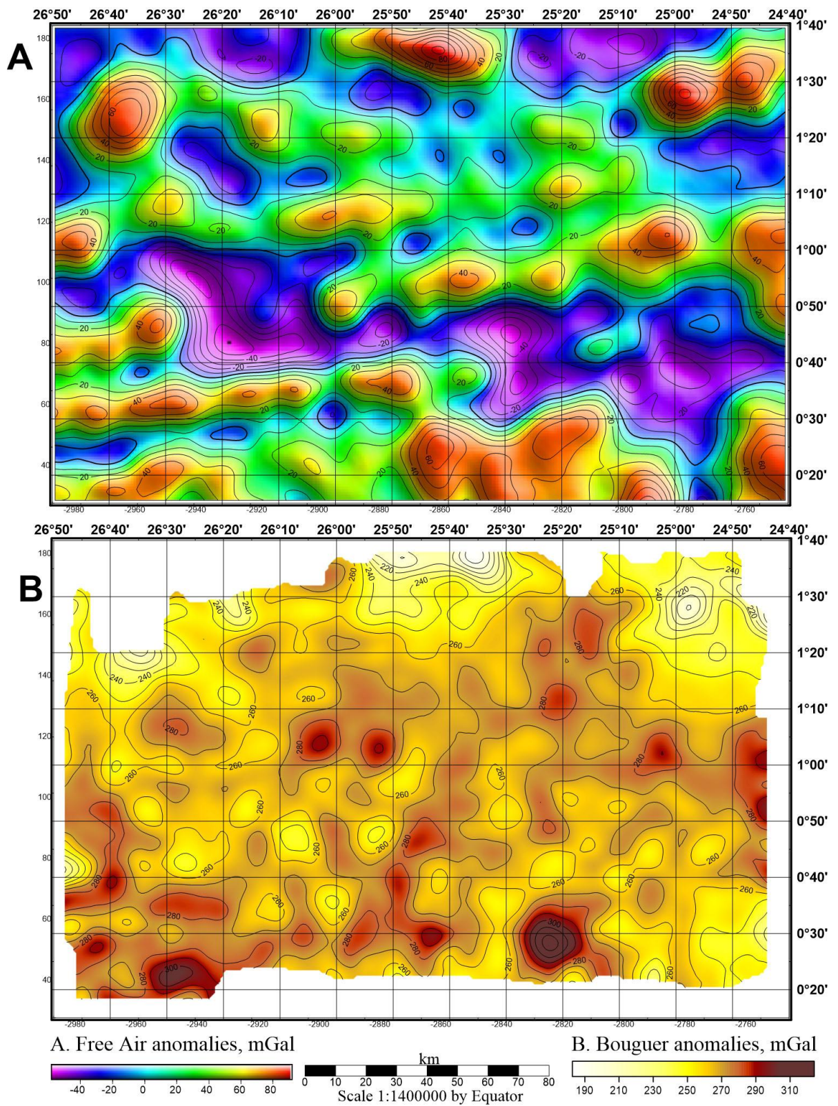
Figure 9. Gravity field over the active segment of the São Paulo FZ. A – free air anomaly; B – Bouguer anomaly.
