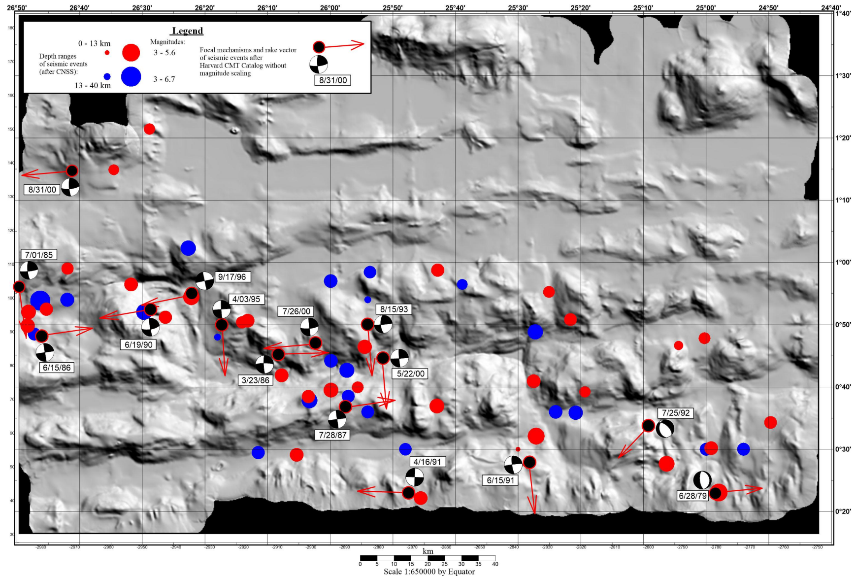
Figure 10. Seismicity of the active segment of the São Paulo FZ.
