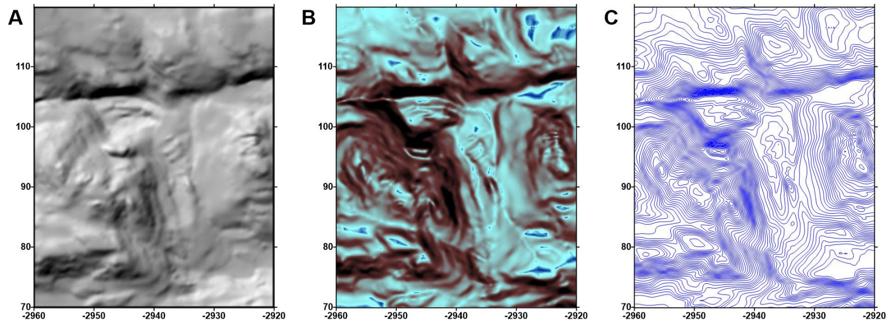
Figure 14. Detailed maps showing the SP2-3_RI rift zone (26°25'W): a - bathymetric map constructed using the shaded relief technique; b - map showing slope angles; c - bathymetric map with a 50-m contour interval. Projection coordinates.
