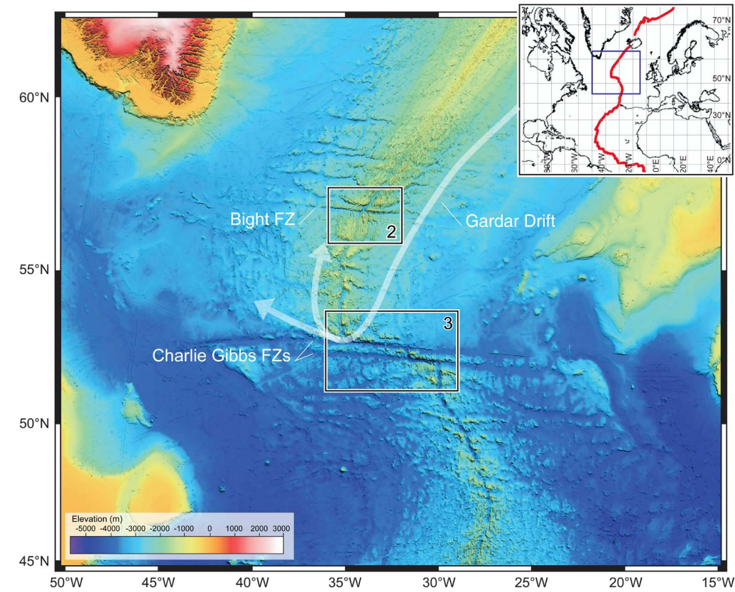
Fig. 1 - Bathymetry of the northern Mid-Atlantic Ridge from the GEBCO_2022 Grid (GEB- CO Compilation Group 2022, doi:10.5285/e0f0bb80-ab44-2739-e053-6c86abc0289c). Location of the Bight and Charlie Gibbs Fracture Zones are indicated. Numbered white boxes indicate Figs. 2 and 3 in this paper, each with bathymetry of specific areas. The inset in the top right corner shows the location of the studied area along the Mid-Atlantic Ridge. White arrows represent Iceland-Scotland Overflow Water.
