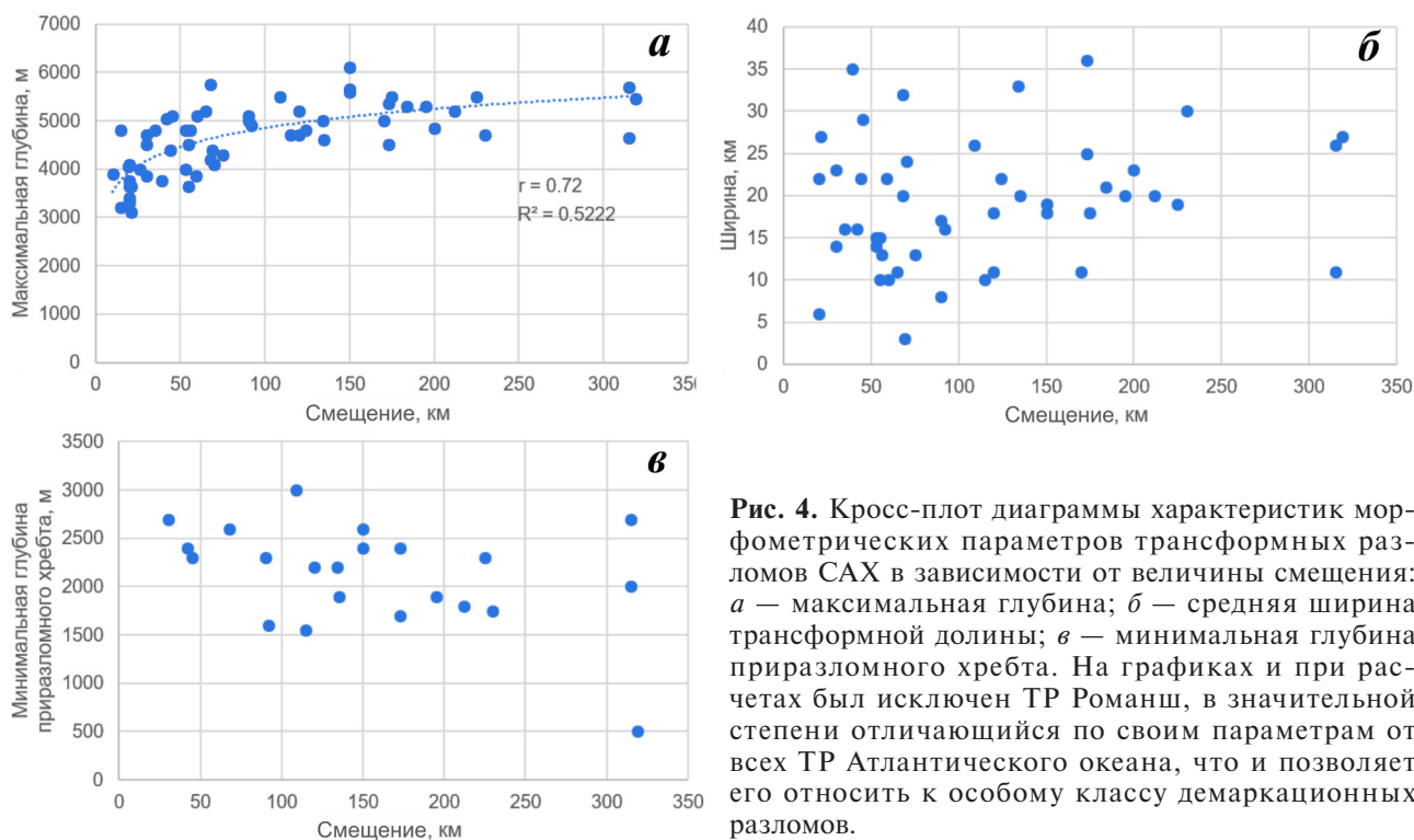
Fig. 4. Cross-plots of transform faults morphometric parameters for MAR depending on offset size: a — maximal depth; б — average width of the transform valley; в — minimal depth of transverse ridge. In the plots and calculations, the TF Romanche, which differs considerably in its parameters from all the TFs of the Atlantic Ocean, was excluded, which allows it to be referred to a special class of demarcation faults.
